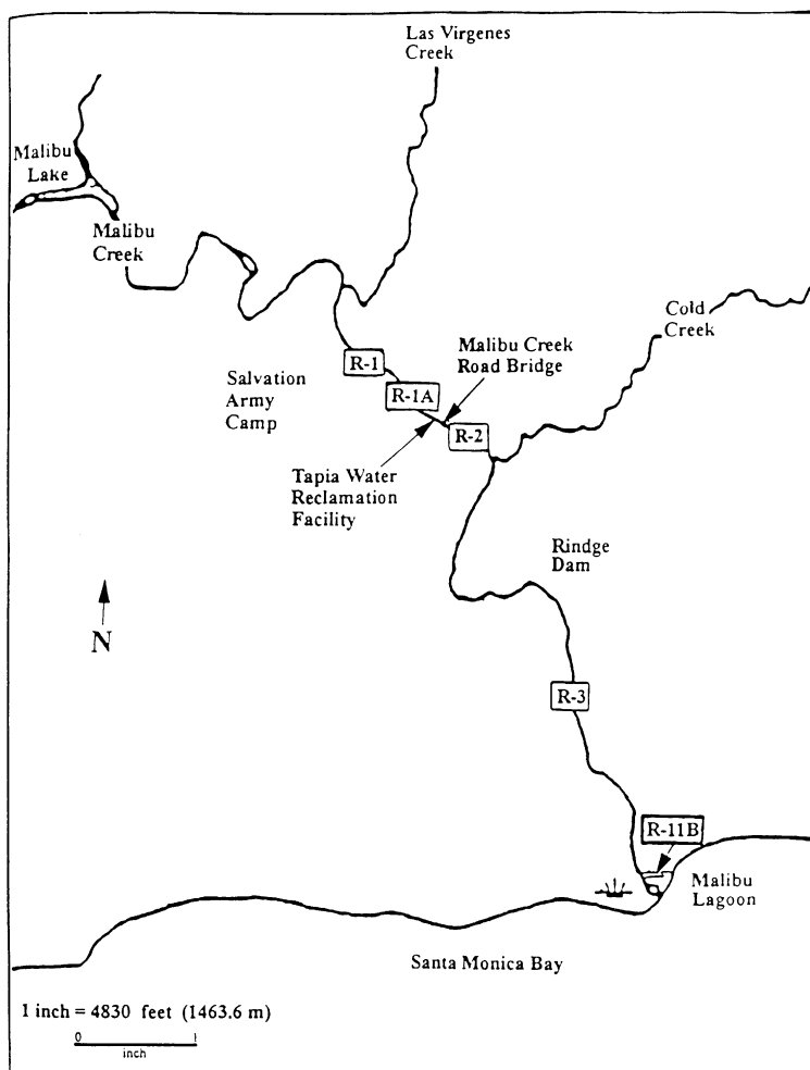
Fig. 1. Map of the Malibu Creek and Malibu Lagoon area showing the location of the sampling stations (R-1, R-1A, R-2, and R-11B).
